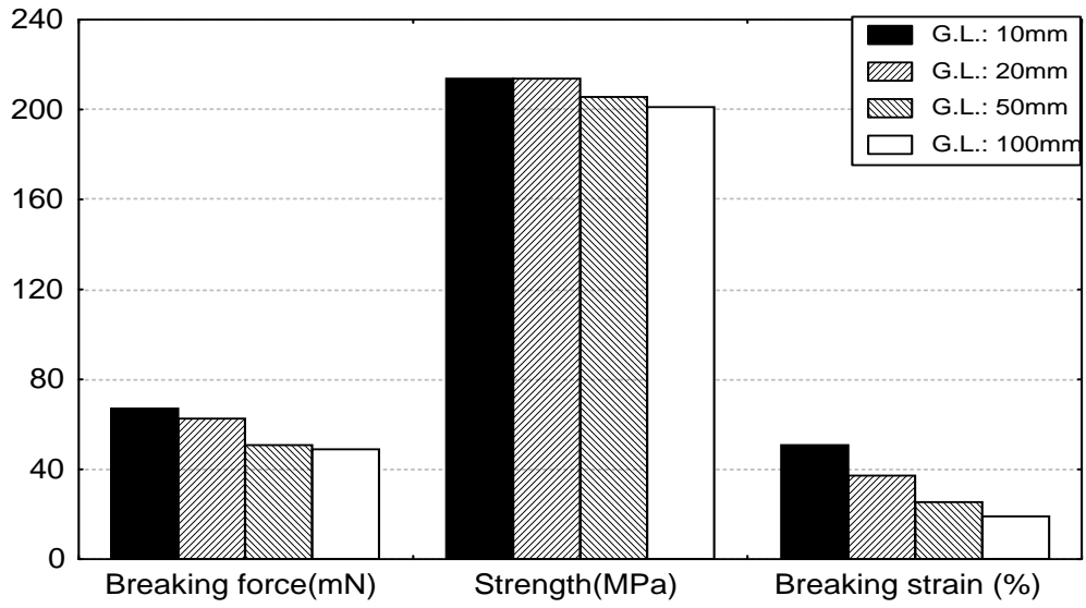
Fig.5 Gauge length effect
