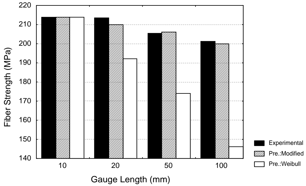
Fig. 6 A comparison between the experimental and the predicted values of average fiber strength (predictions are based on the results at 10 mm gauge length)
