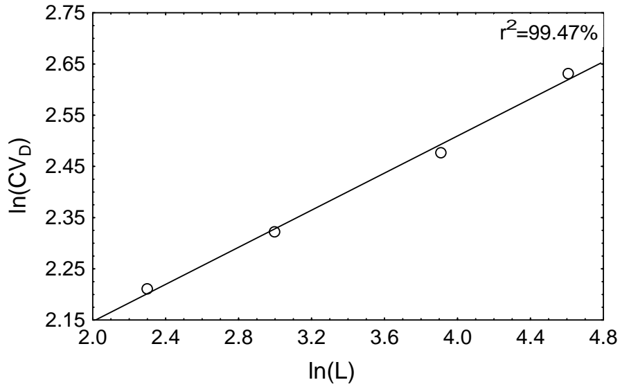
Fig. 2 Change of within-fiber diameter variation with the gauge length
