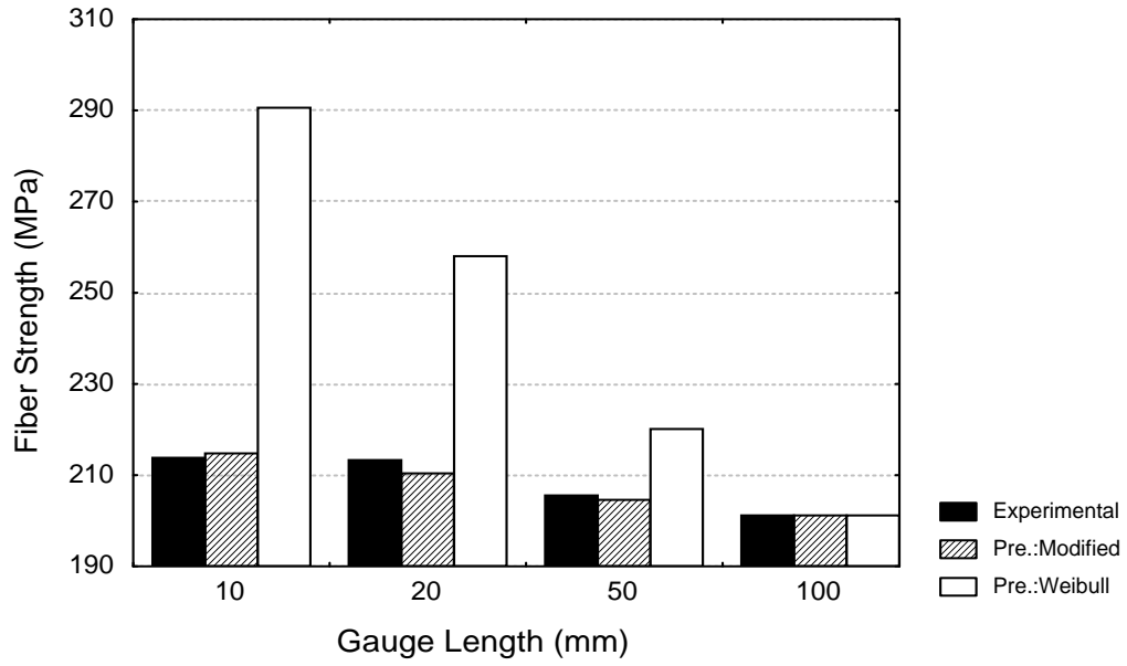
Fig. 7 A comparison between the experimental and the predicted values of average fiber strength (predictions are based on the results at 100 mm gauge length)
