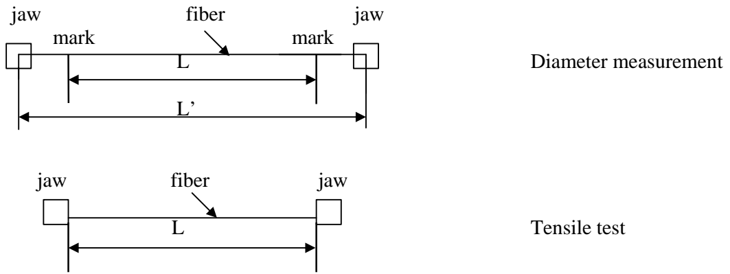
Fig. 1: A diagram illustrating the diameter and tensile tests
