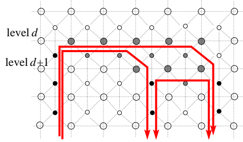
Figure 3: Decomposition with respect to symmetric/asymmetric Markov blankets.
