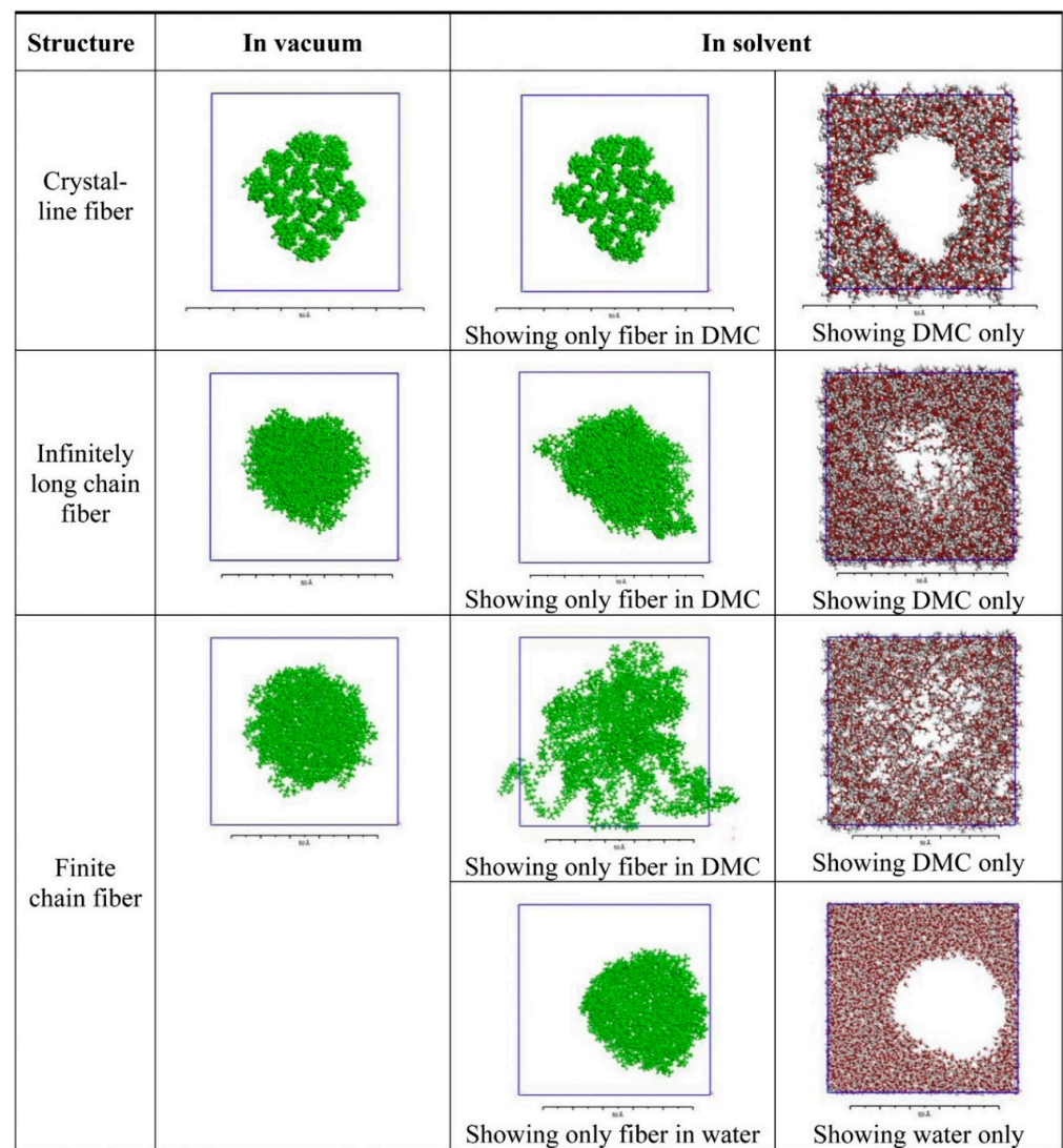
Figure 5. Relaxed structure for crystalline fibre, infinitely long chain fibre and finite chain fibre in vacuum, in DMC, and in water at zero strain [43].
