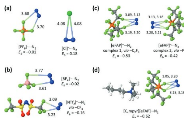
Fig. 3 (a–c) N_2 binding energies (in kcal\ mol^{-1} ) and bond distances in \text{\AA} for various anions. The interaction with [eFAP]^- in panel (c) shows two distinct modes: complex 1 exhibits C–F interactions and complex 2, P–F interactions. Panel (d) introduces the cation to show the interaction with an ion pair of [C_4mpyr][eFAP] ; the interaction is the strongest of all those studied.
