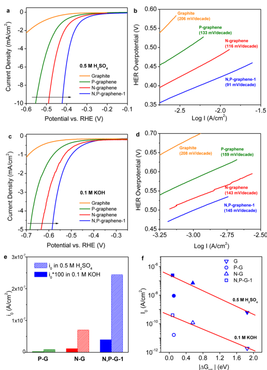
Figure 3. HER polarization curves and the corresponding Tafel plots of N- and/or P-doped graphene electrocatalysts in (a, b) 0.5 M \text{H}_2\text{SO}_4 (pH = 0) and (c, d) 0.1 M KOH (pH = 13). (e) Comparison of calculated i_0 values for N- and/or P-doped graphenes in 0.5 M \text{H}_2\text{SO}_4 (patterned bars) and 0.1 M KOH (solid bars) solutions. (f) Relationships between i_0 and \Delta G_{\text{H}^*} for N- and/or P-doped graphenes.
