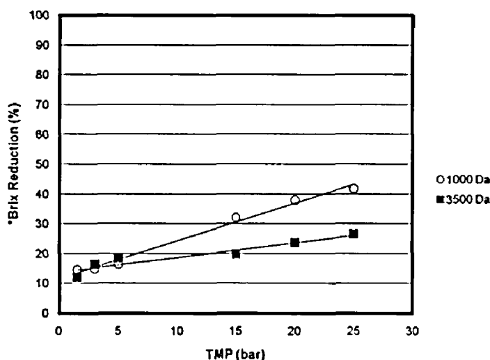
Fig. 7 Graph of mean °Brix reduction at different TMP for 1000 and 3500 Da membranes at pH 7.5
