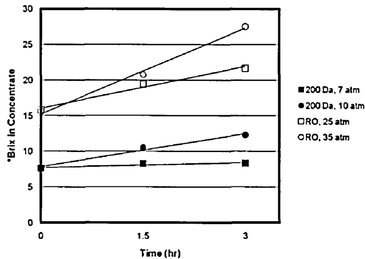
Fig. 8 Graph of mean °Brix in concentrate for 200 Da and RO membranes at various operating times and pressures
