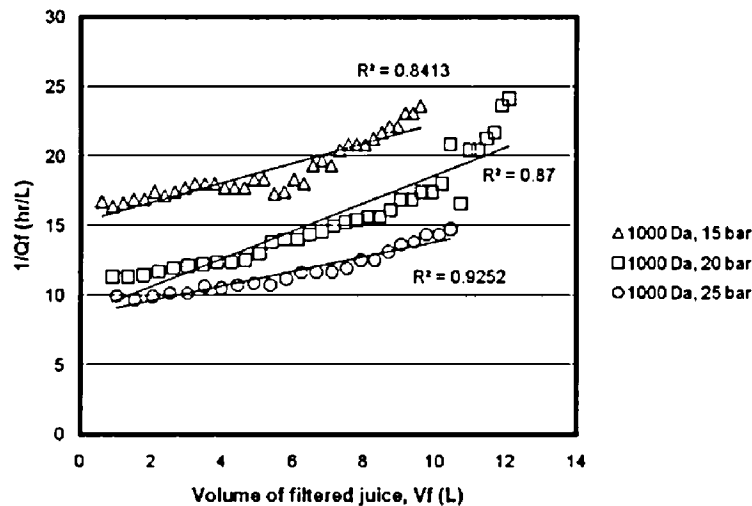
Fig. 5 Graph of combination of external and progressive internal fouling model fitting to the experimental data for 1000 Da membrane at temperature of 35°C and pH 7.5
