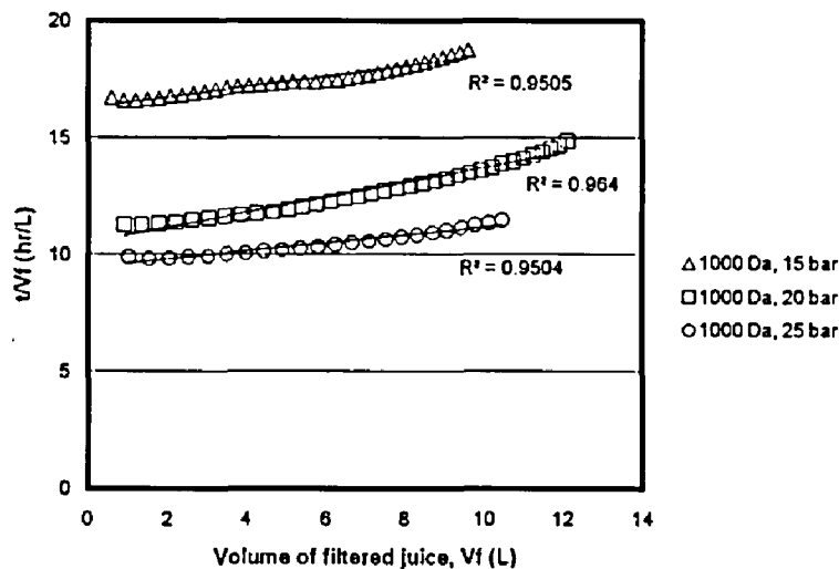
Fig. 3 Graph of cake filtration model fitting to the experimental data for 1000 Da membrane at temperature of 35°C and pH 7.5
