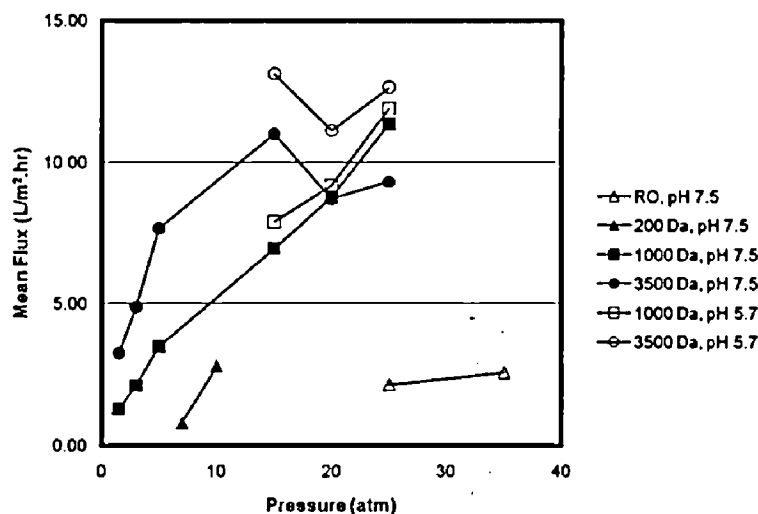
Fig. 2 Graph of overall mean flux for each membrane at different operating pressures and pH
