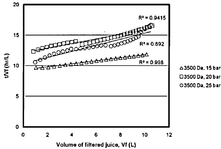
Fig. 4 Graph of cake filtration model fitting to the experimental data for 3500 Da membrane at temperature of 35°C and pH 7.5
