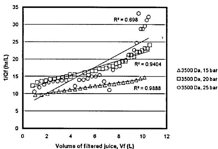
Fig. 6 Graph of combination of external and progressive internal fouling model fitting to the experimental data for 3500 Da membrane at temperature of 35°C and pH 7.5
