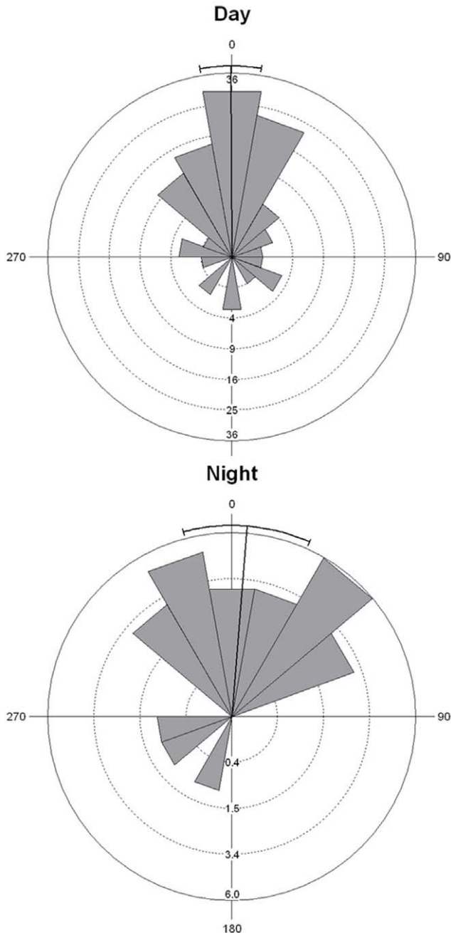
Figure 4. Rose diagrams showing the angular changes of N. cepedianus for both day and night periods. Note differences in scale between the two periods.
