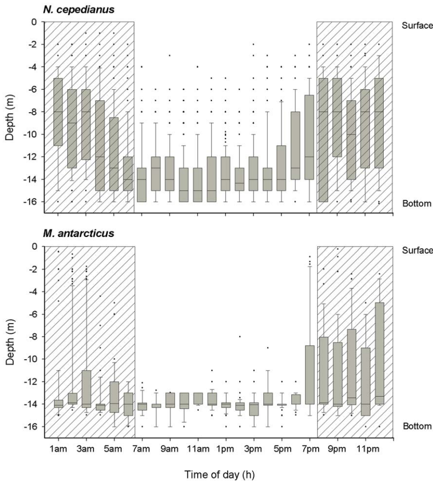
Figure 2. Diel pattern in depth use for N. cepedianus and M. antarcticus in southeast Tasmania. Box plots show the median (line within the boxes), interquartile ranges (boxes), 10 th and 90 th percentiles (whiskers) and outliers (+) of depths detected during each 1 h interval. For each species, data from the whole sampling period was pooled. Dashed area indicates nocturnal period. doi:10.1371/journal.pone.0015464.g002
