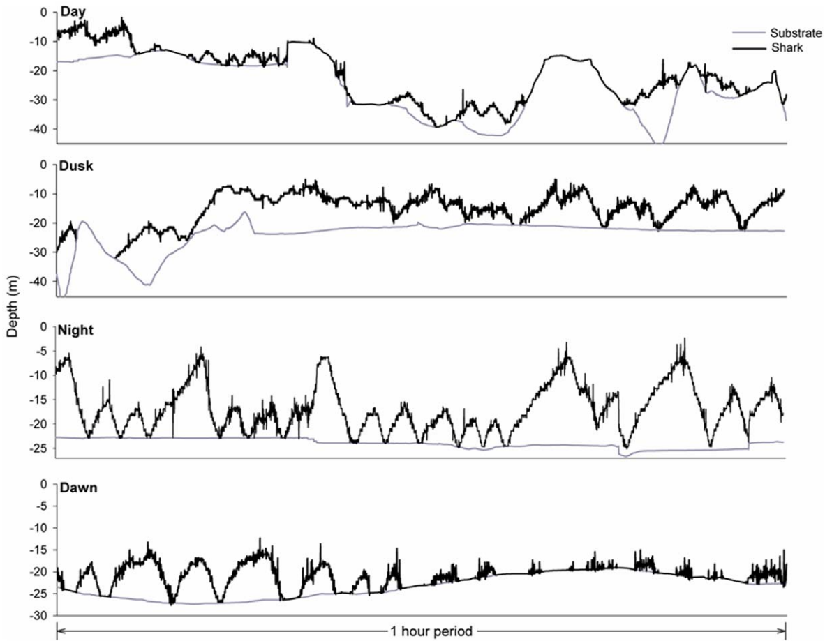
Figure 5. Typical depth profiles for each of the different periods of the diel cycle. Data illustrates the profile over representative 1 h periods during the day (16:00–17:00 h), dusk (20:00–21:00 h), night (01:00–02:00 h) and dawn (05:00–06:00 h) periods for the N. cepedianus individual tracked in the Derwent Estuary on the 16 th March 2007. doi:10.1371/journal.pone.0015464.g005
