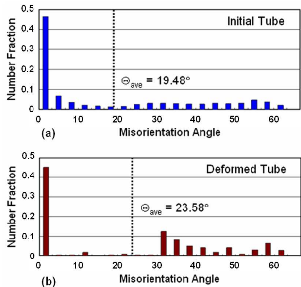
Fig. 5 Distribution of misorientation angle of (a) initial tube, (b) deformed tube
