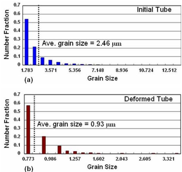
Fig. 4 Distribution of grain size of (a) initial tube, (b) deformed tube
