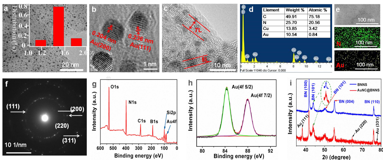
Figure 1. Typical TEM images of AuNC@BNNSs nanohybrid with different magnifications, XPS and XRD spectra. (a) Low-magnification TEM image of AuNC@BNNSs. The inset shows the size distribution of AuNCs. (b) High-magnification TEM image showing the single crystalline structure and multi-crystalline structure of AuNCs. (c) HRTEM image of BNNSs with clear latticefringes. (d) EDX spectrum of AuNC@BNNSs nanohybrid and the relative abundance of each element. (e) The elemental mappings of N and Au. (f) SAED pattern of AuNC@BNNSs. (g) Survey XPS spectrum of AuNC@BNNSs. (h) Au 4f narrow XPS scan spectra. (i) XRD patterns of BNNSs and AuNC@BNNSs.
