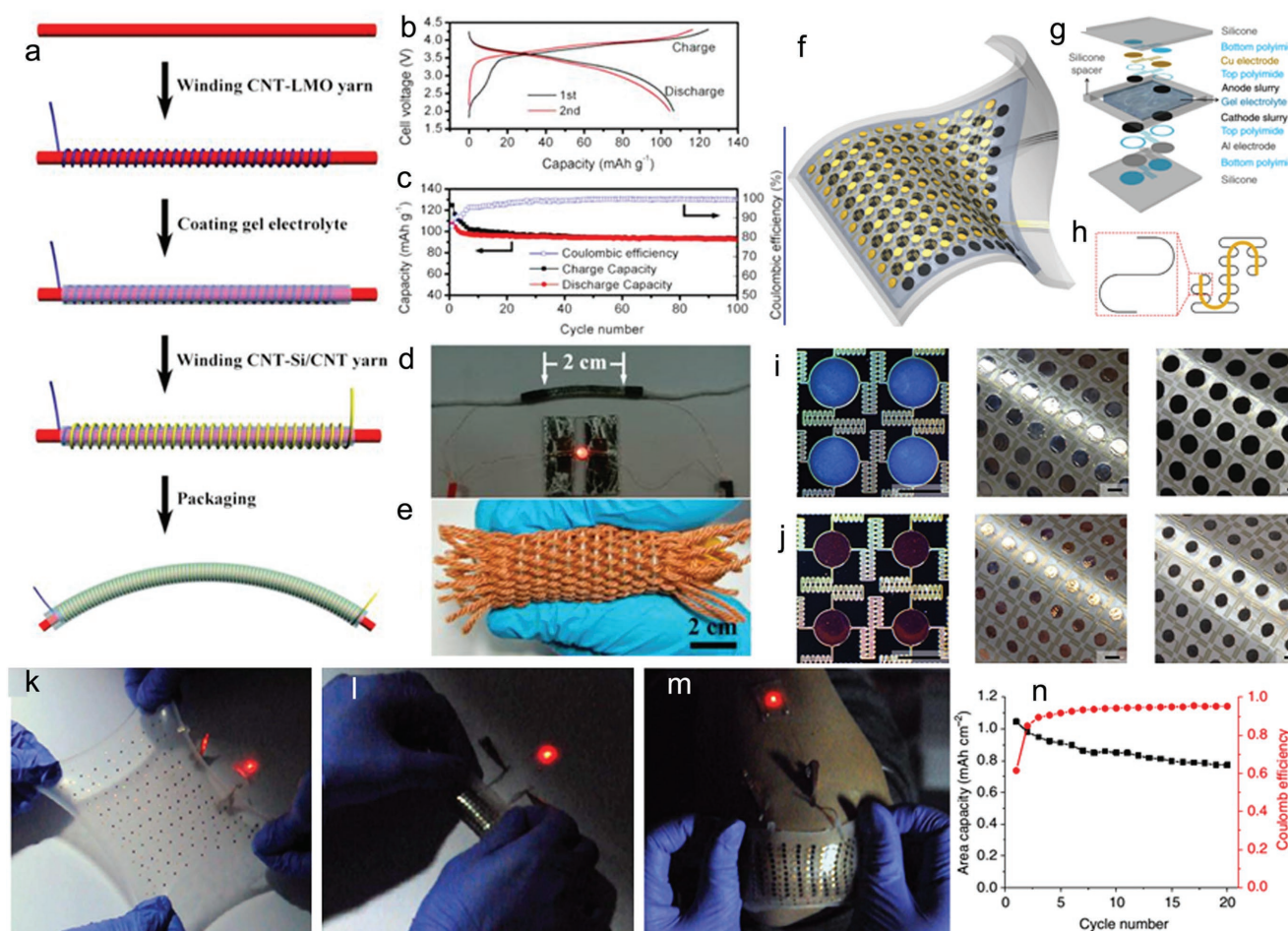
Figure 12. a) Schematic of the fabrication process based on the coaxial fiber full LIB. b) Voltage profiles and c) long-life performance of the fiber-shaped LIB. d) Photograph of the fiber-shaped LIB to power a light emission diode. e) The fiber-shaped full LIBs being woven into a textile. f) Schematic illustration of a completed stretchable device. g) Exploded view layout of the various layers in the battery structure. h) Illustration of “self-similar” serpentine geometries used for the interconnects. Optical images of i) the Al electrode pads and self-similar interconnects on a Si wafer and j) the Cu electrode pads and self-similar interconnects on a Si wafer. Operation of a battery connected to a red light-emitting diodes (LED) while k) biaxially stretched to 300%, l) folded, and m) mounted on the human elbow. n) Capacity retention (black) and coulombic efficiency (red) of the stretchable device over 20 cycles. a–e) Reproduced with permission. [132] Copyright 2014, American Chemical Society. f–n) Reproduced with permission. [133] Copyright 2013, Nature Publishing Group.
