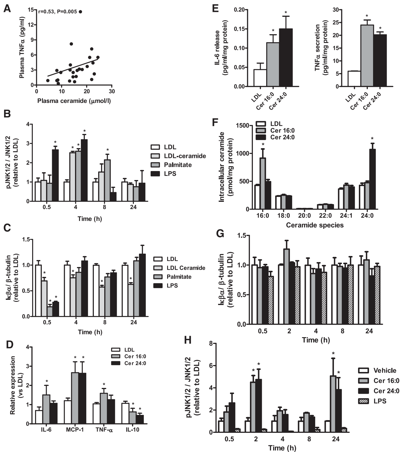
FIG. 5. LDL-ceramides contribute to an M1 phenotype in cultured macrophages. Relationship between plasma ceramide and plasma \text{TNF}\alpha from age-matched lean, insulin-sensitive ( n = 10 ); obese, insulin-sensitive ( n = 5 ); and obese, type 2 diabetic individuals ( n = 10 ). B and C : RAW 264.7 macrophages were incubated with LDL, 100 nmol/L LDL-ceramide, 100 ng/mL LPS, or 0.75 mmol/L palmitate for the indicated time. Cells were lysed and assessed for JNK phosphorylation ( B ) or \text{I}\kappa\text{B}\alpha ( C ) by immunoblot analysis. n = 3 per group. *P < 0.05 vs. LDL by one-way ANOVA and Tukey post hoc analysis. Representative blots can be found in Supplementary Fig. 6. D : Cells were treated with LDL or LDL-ceramide for 24 h. RNA was extracted and reverse transcribed, and mRNA content was assessed by quantitative RT-PCR. All data were normalized to 18S. n = 9 per group. *P < 0.05 vs. LDL by unpaired Student t test. E : Cells were treated with LDL or LDL-ceramide for 24 h and washed, and the culture medium was replaced with no additions. The medium was collected after 24 h, and \text{TNF}\alpha and IL-6 were analyzed by ELISA. n = 3 per group. *P < 0.05 vs. LDL by unpaired Student t test. F : Macrophages were treated with LDL or LDL-ceramide for 24 h, cells were lysed, lipids were extracted, and ceramide species were quantified by mass spectrometry. n = 6 per group. *P < 0.05 vs. LDL by unpaired Student t test. G and H : MyD88 -/- / Ticam1 -/- macrophages were incubated with LDL, 100 nmol/L LDL-ceramide, or 100 ng/mL LPS for the indicated time. Cells were lysed and assessed for \text{I}\kappa\text{B}\alpha levels ( G ) or JNK phosphorylation ( H ) by immunoblot analysis. n = 3 per group. *P < 0.05 vs. LDL. All data are presented as means \pm SEM by one-way ANOVA and Tukey post hoc analysis. Representative blots can be found in Supplementary Fig. 6.
